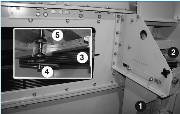
Drive system with external motor
